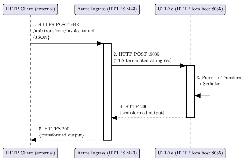
Figure 3: Scenario 3: Direct HTTP via Azure ingress, no Dapr
