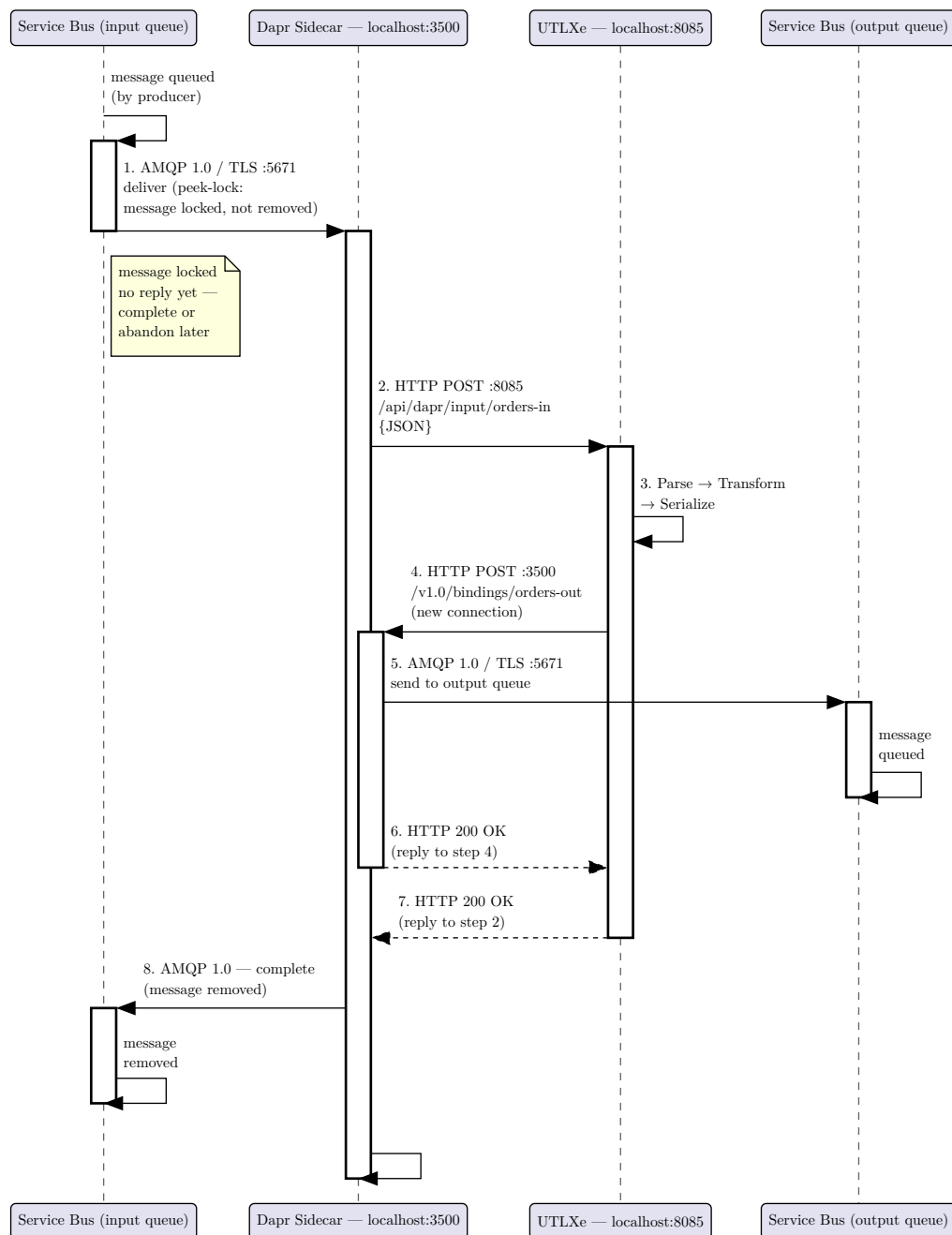
Figure 1: Scenario 1: Azure Service Bus queue-to-queue via Dapr sidecar
